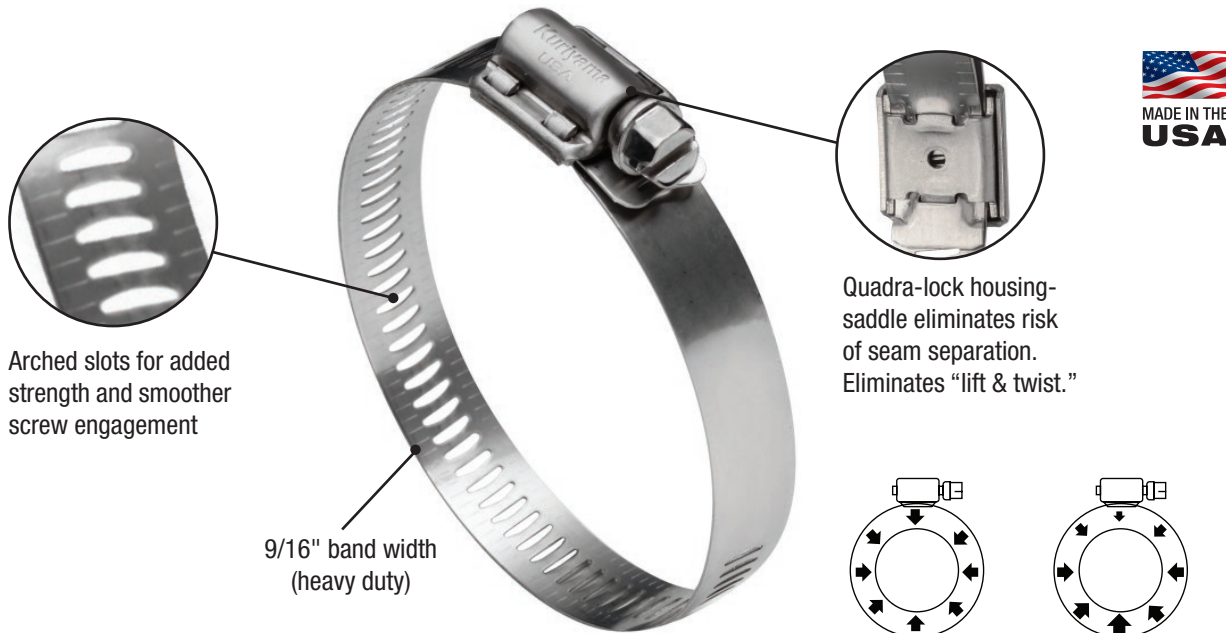
Kuri-Clamp™
