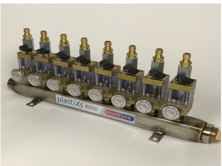
Stainless Steel Manifold Assembly with Flowmeters with Temperature Gauges, Mini Ball Valves, and Quick Connect Plugs
