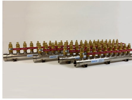
1 1/2" Special Compact Stainless Steel Manifold Assemblies with Full Port Brass Ball Valves and a Unique Pre-Threaded Mounting System
