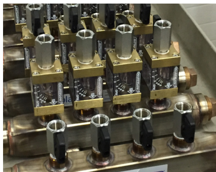
Supply and Return Manifold Pair Assemblies with Mini Ball Valves and Mechanical Flowmeters on the Return Side for Injection Molding Application
