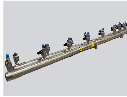
Large Custom Stainless Steel Manifold Assembly for Cooling Drive on Semiconductor Equipment
