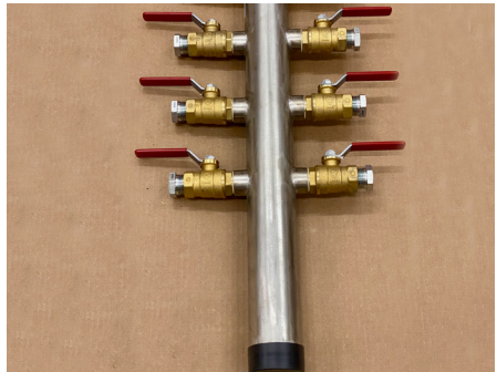
Custom Stainless Steel Manifold Assembly with 180° Ports Installed with Full Port Ball Valves for Welding Gases in an Automotive Frame Assembly Plant
